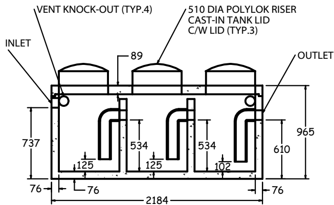
SIDE SECTION 1:40
