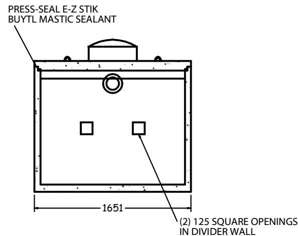
END SECTION 1:40
