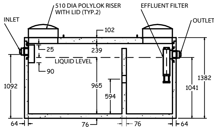
SIDE SECTION 1:40
