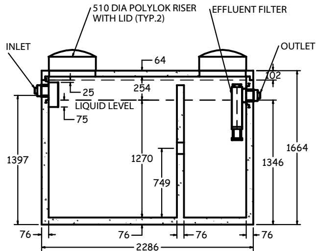
SIDE SECTION 1:40
