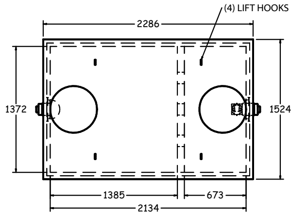
TOP VIEW 1:40
