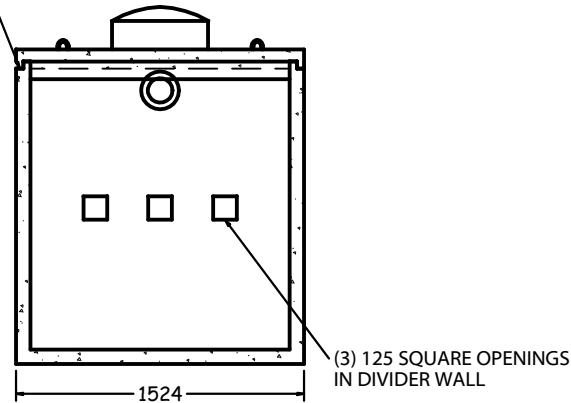
END SECTION 1:40
