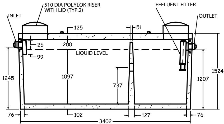
SIDE SECTION 1:40
