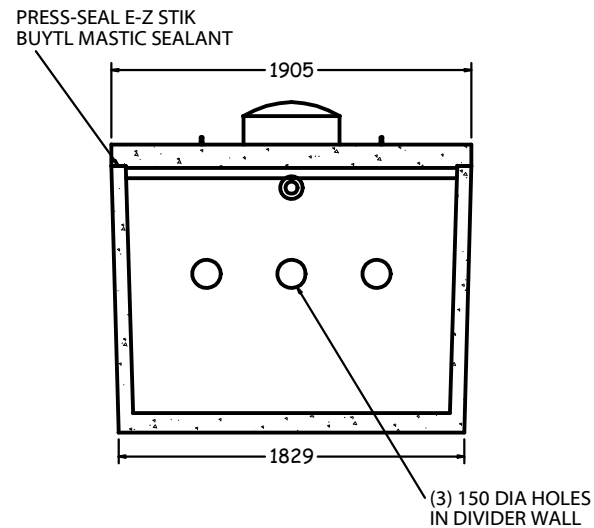
END SECTION 1:40
