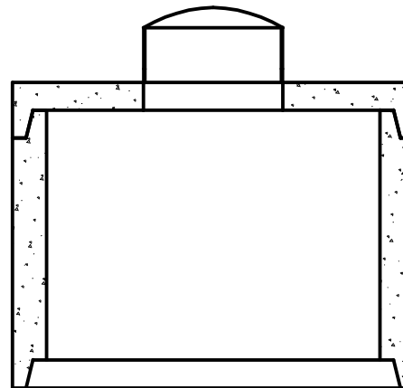
FRONT SECTION 1:25
