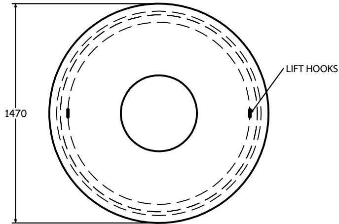
TOP VIEW 1:25
