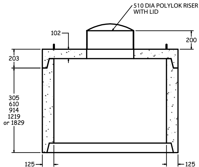
SIDE SECTION 1:25
