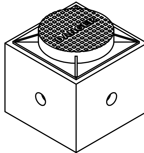
ISOMETRIC VIEW 1:20
