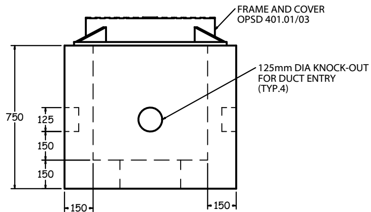
FRONT VIEW 1:20
