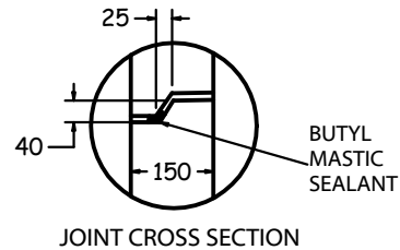
JOINT CROSS SECTION
