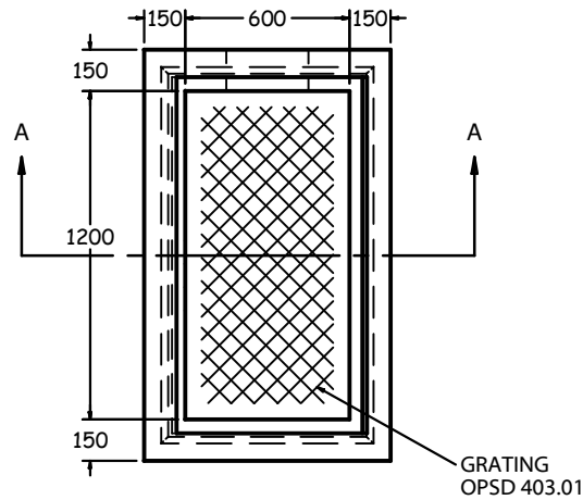
TOP VIEW 1:30
