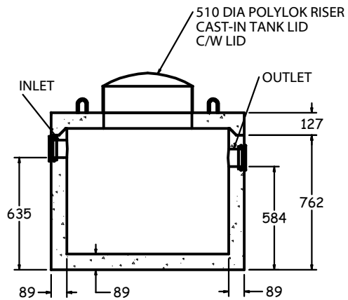
FRONT VIEW 1:30
