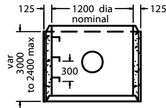
SECTION E-E RISER SECTION
