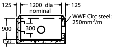
SECTION C-C MONOLITHIC BASE
