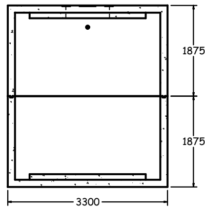
END SECTION 1:80
