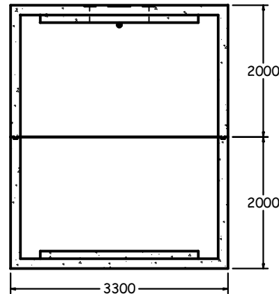
END SECTION 1:80
