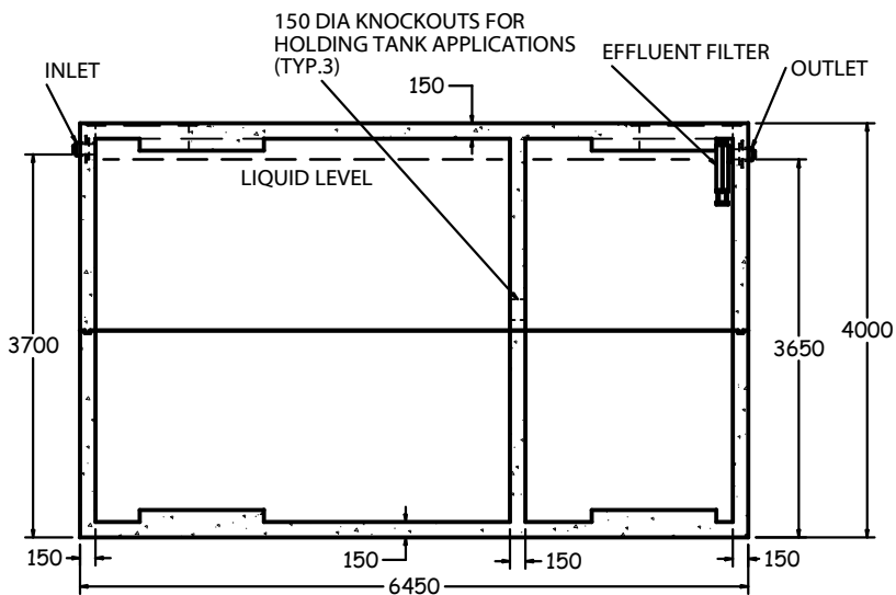
SIDE SECTION 1:80
