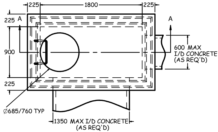
TOP VIEW 1:40
