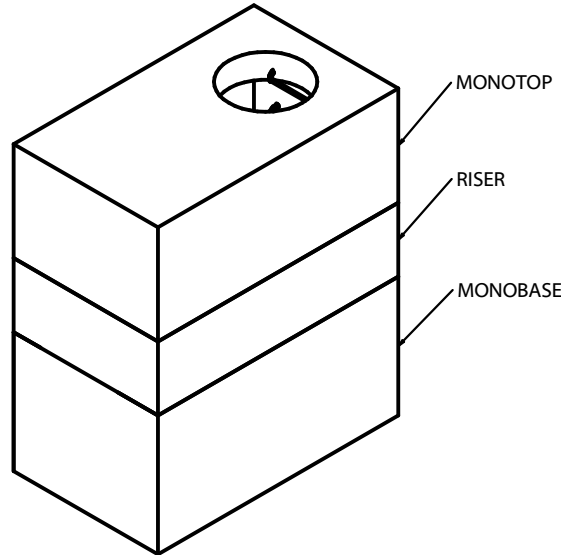
ISOMETRIC VIEW 1:50
