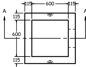
TOP VIEW 1:30
