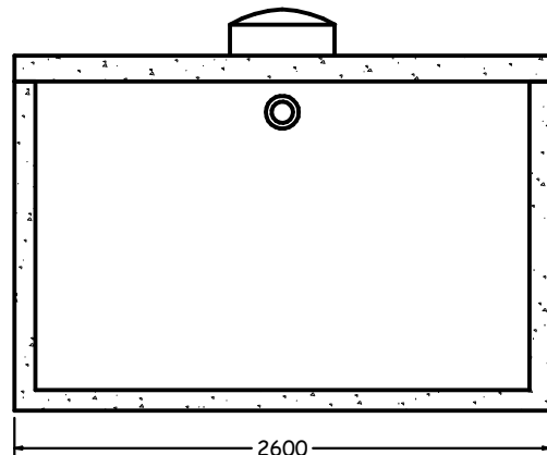
END SECTION 1:40
