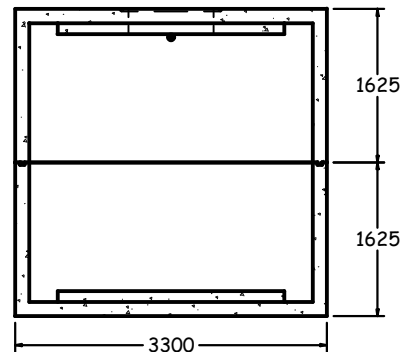
END SECTION 1:80
