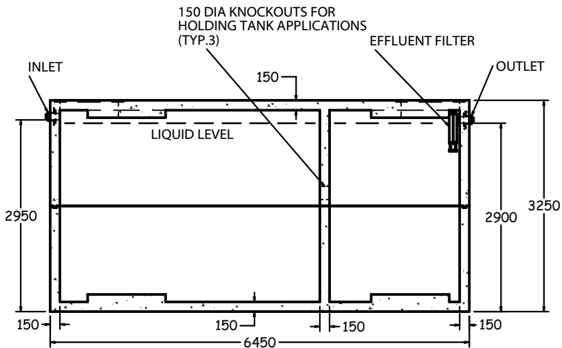
SIDE SECTION 1:80
