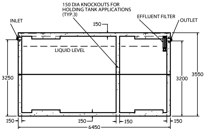
SIDE SECTION 1:80
