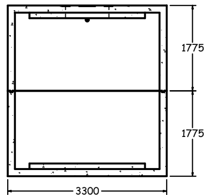
END SECTION 1:80
