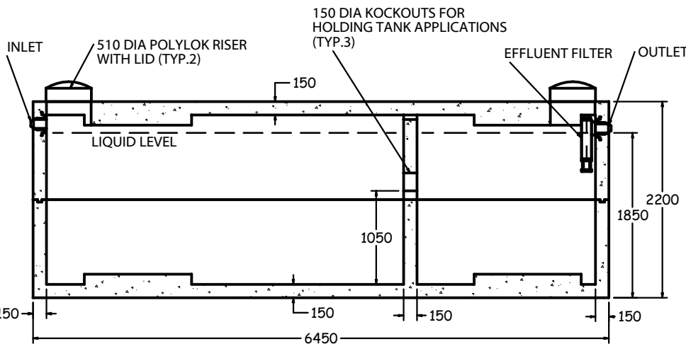
SIDE SECTION 1:60
