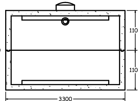
END SECTION 1:60
