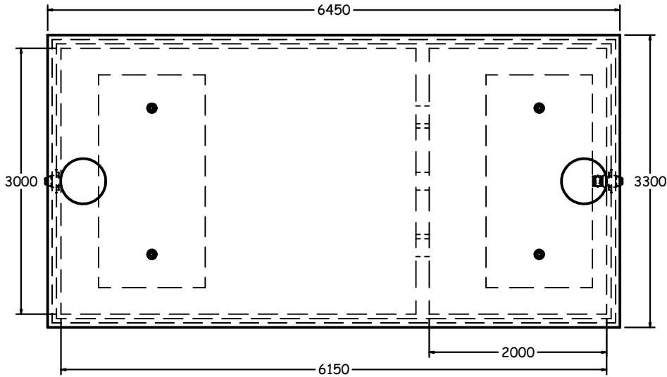
TOP VIEW 1:60
