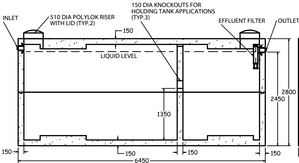
SIDE SECTION 1:60
