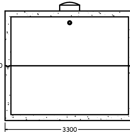
END SECTION 1:60
