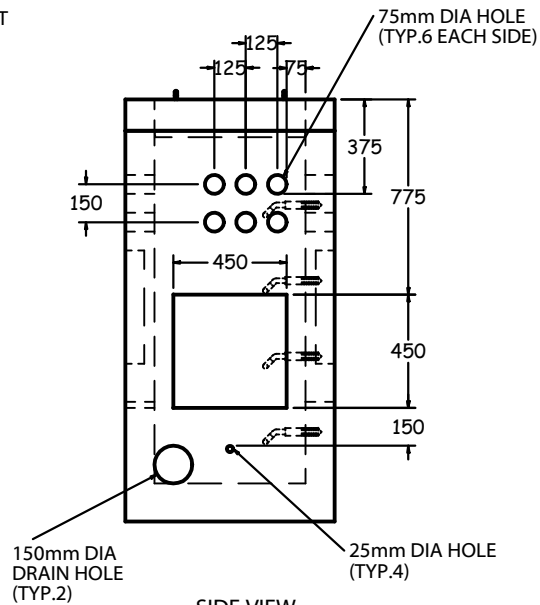
SIDE VIEW 1:30
