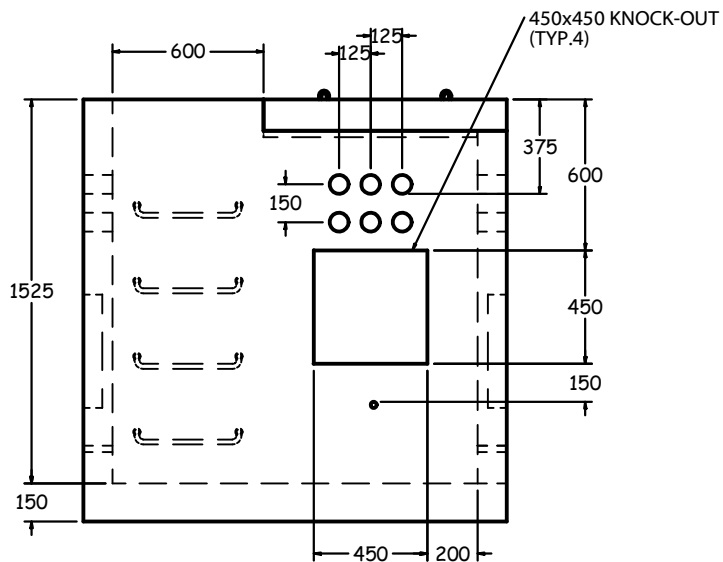
FRONT VIEW 1:30
