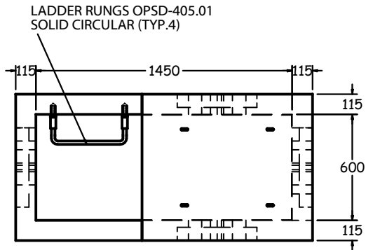
TOP VIEW 1:30
