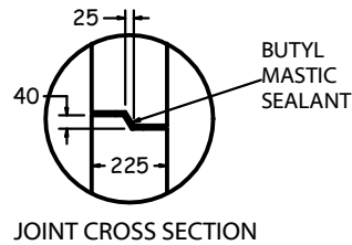
JOINT CROSS SECTION
