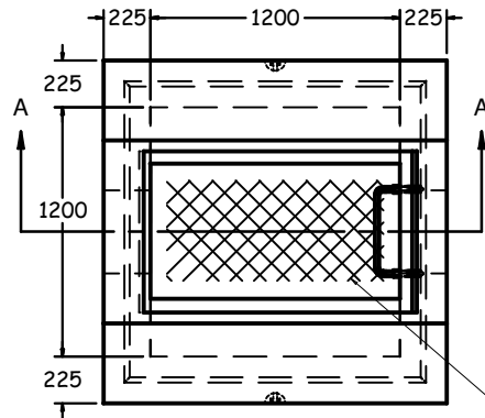
TOP VIEW 1:40
